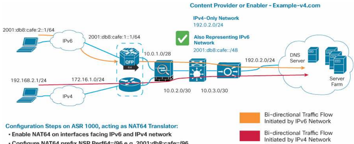
Figure 10. Providing Existing Services to the IPv6 Internet
