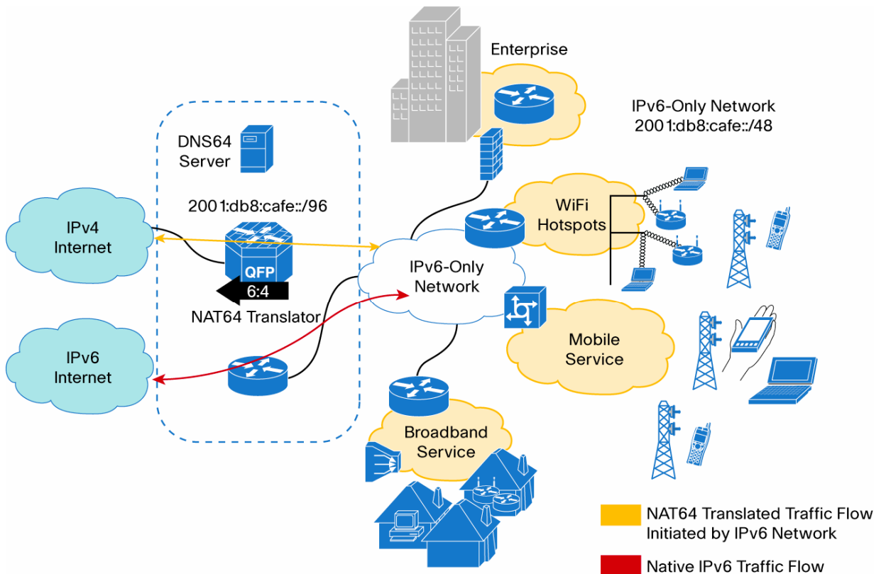
Figure 4. Greenfield IPv6-Only Network
