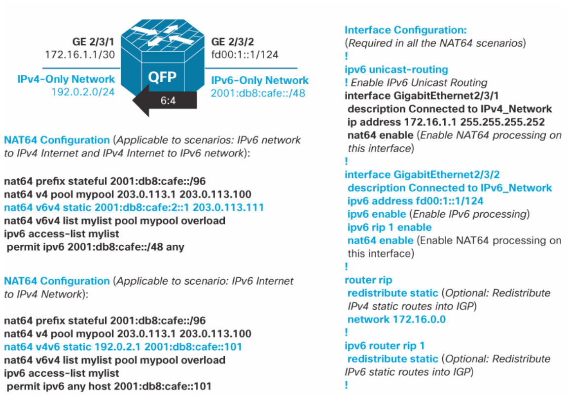
Figure 17. Configuration for Stateful NAT64 Translation
