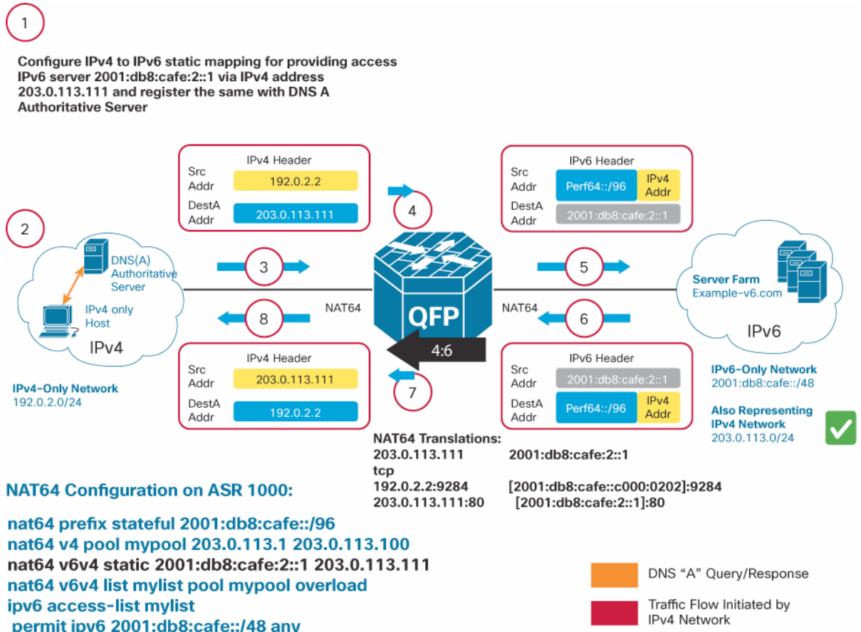
Figure 15. Cisco ASR 1000 Series Router Translating IPv4 Traffic to IPv6 and IPv6 Traffic to IPv4
